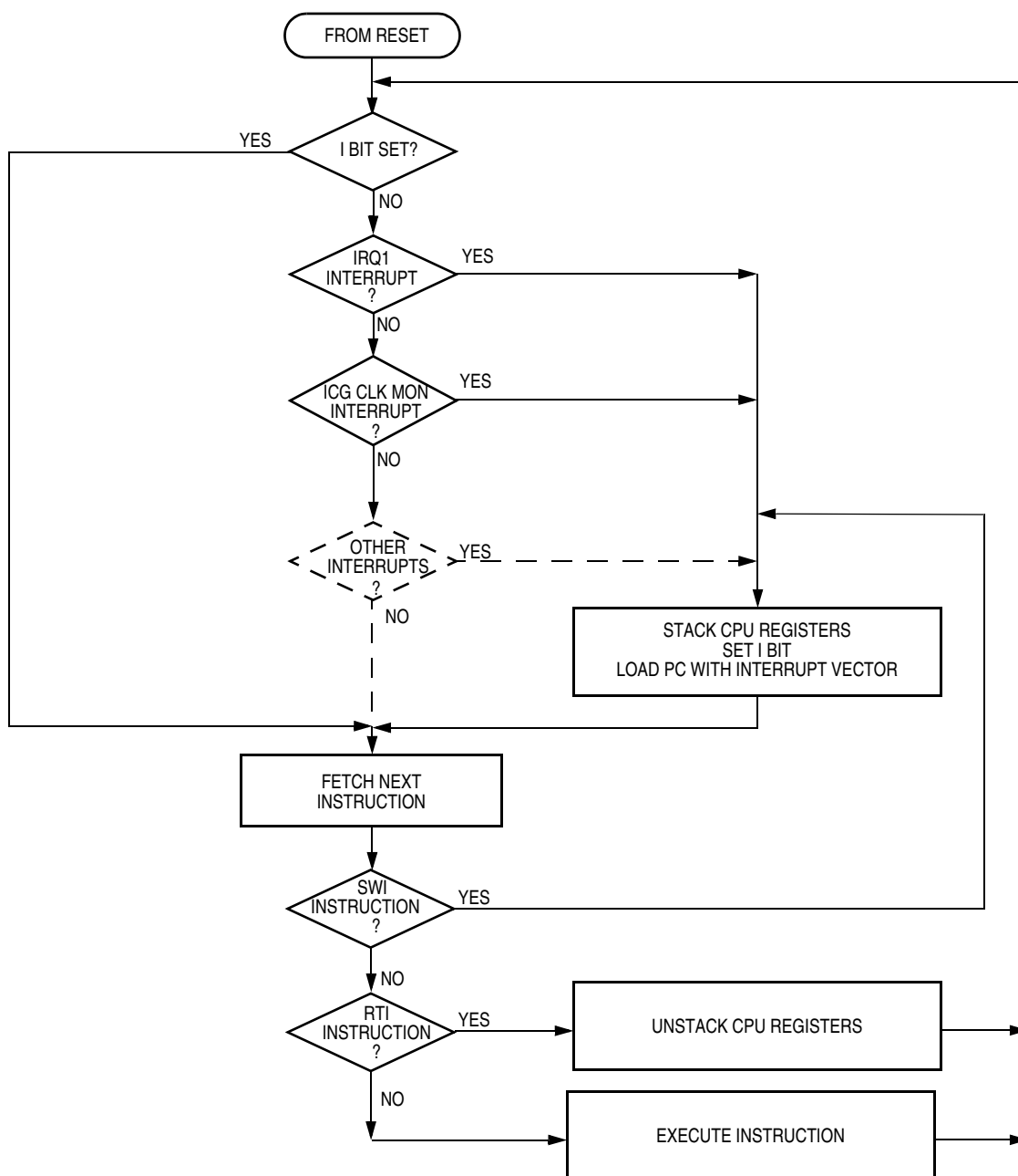
Figure 13-9. Interrupt Processing
