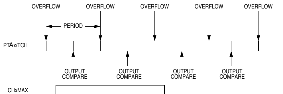
Figure 15-9. CHxMAX Latency
