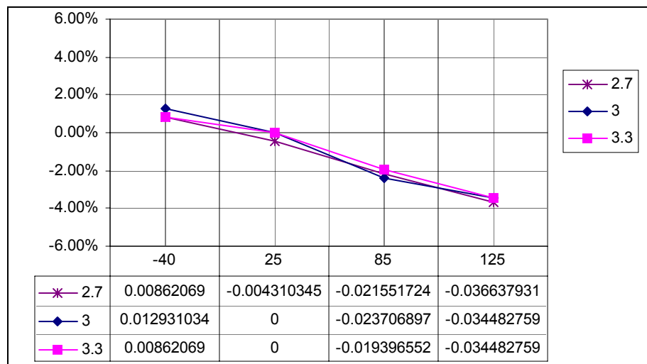
Figure 17-1. Example of Frequency Variation Across Temperature, Trimmed at Nominal 3 Volts, 25°C, and N = 1
