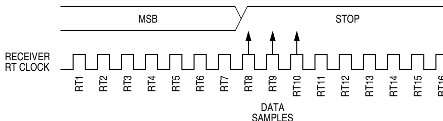
Figure 12-8. Slow Data
