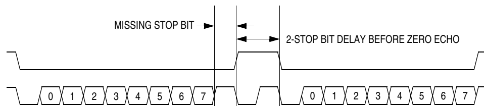
Figure 16-11. Break Transaction
