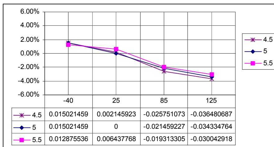
Figure 17-3. Example of Frequency Variation Across Temperature, Trimmed at Nominal 5 Volts, 25°C, and N = 1
